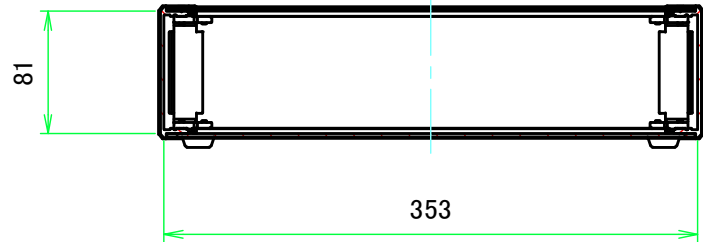
B-B (1:5)
